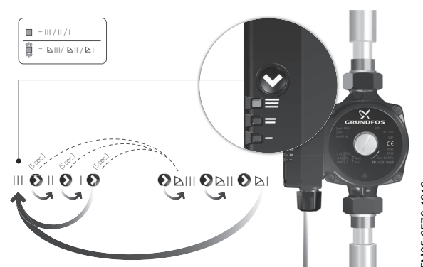
Fig. 13 Control modes
